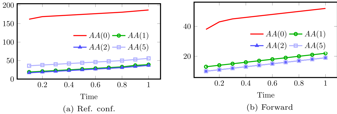
Fig. 7. Test 5, Number of accumulated time iterations incurred to solve the (a) IPP and (b) DPP at each ramp step. In (b), the AA(2) and AA(5) lines overlap.
