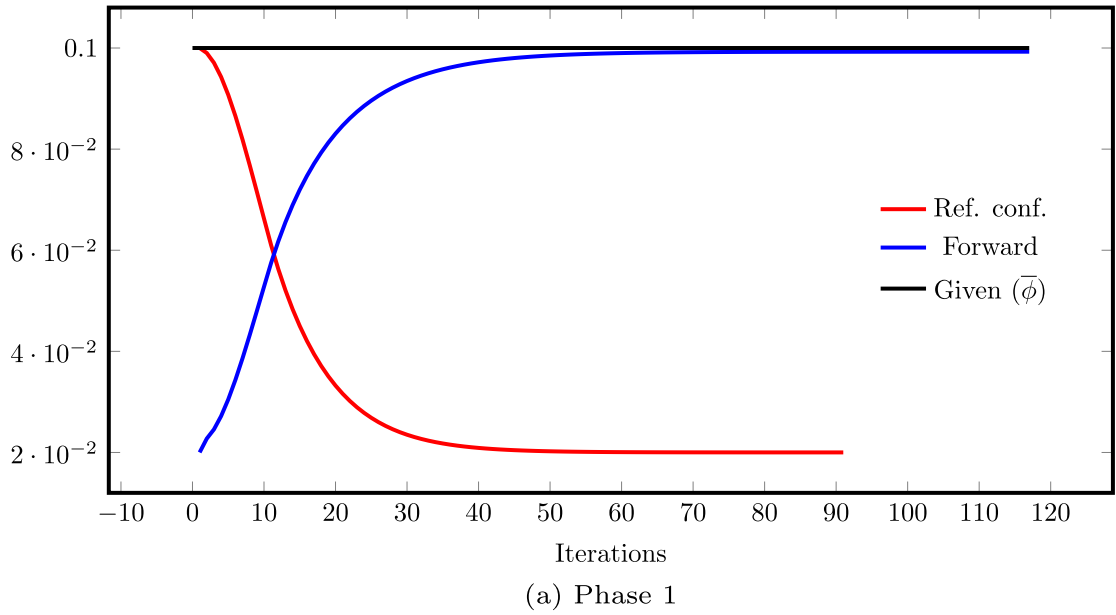
Fig. 4. Test 2, Evolution of the average spatial porosity \frac{1}{|\Omega|} \int_{\Omega} \phi dx along the iterations of both the IPP and DPP in both phases for the brick 3D geometry. The given value \bar{\phi} is shown for comparison.
