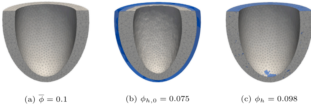
Fig. 6. Test 5, The average Eulerian steady state porosities in the caption for the (a) given geometry, (b) computed reference configuration with the given geometry in a translucent blue, and (c) the deformed geometry from the given loads with the given geometry in a translucent blue. The ‘h’ subscript shows that the function is a FEM approximation. (For interpretation of the references to colour in this figure legend, the reader is referred to the web version of this article.)
