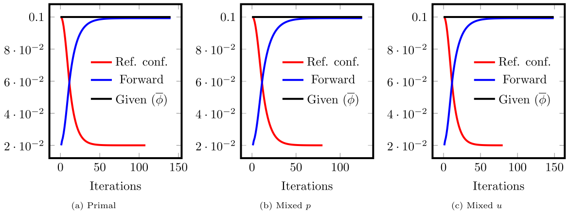
Fig. 5. Test 4, Evolution of the average spatial porosity \frac{1}{|\Omega|} \int_{\Omega} \phi dx along the iterations of both the IPP and DPP. We show the evolution obtained using the (a) primal formulation, (b) the mixed pressure formulation and (c) the mixed velocity formulation.
