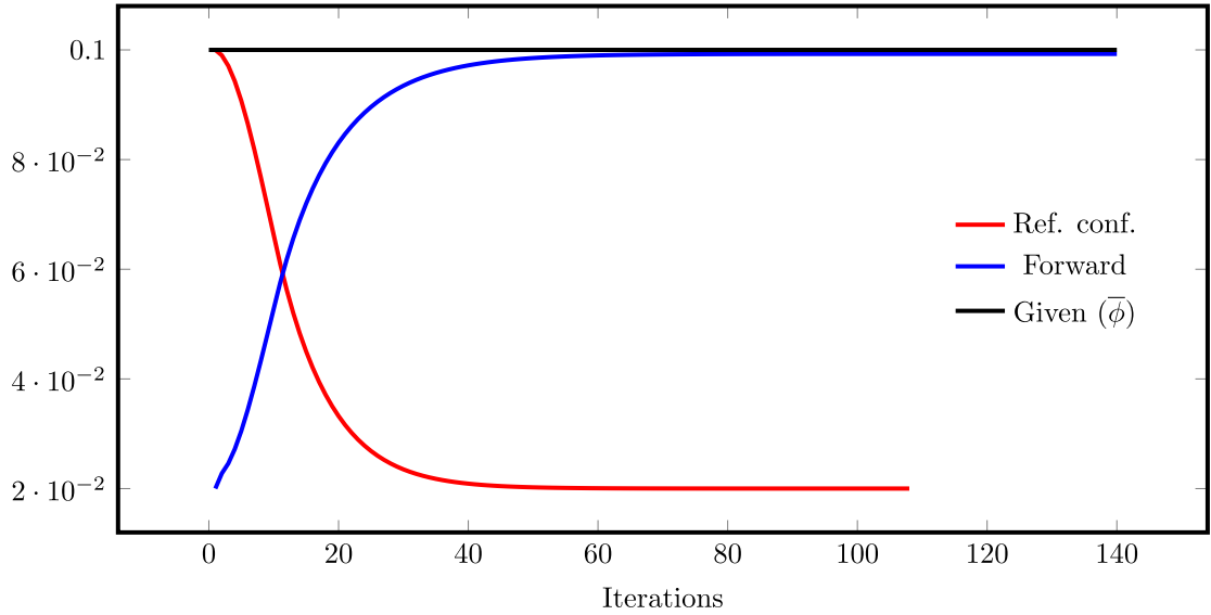
Fig. 2. Test 1, Evolution of the average spatial porosity \frac{1}{|\Omega|} \int_{\Omega} \phi dx along the iterations of both the forward and inverse problems. The given value \bar{\phi} is shown for comparison.
