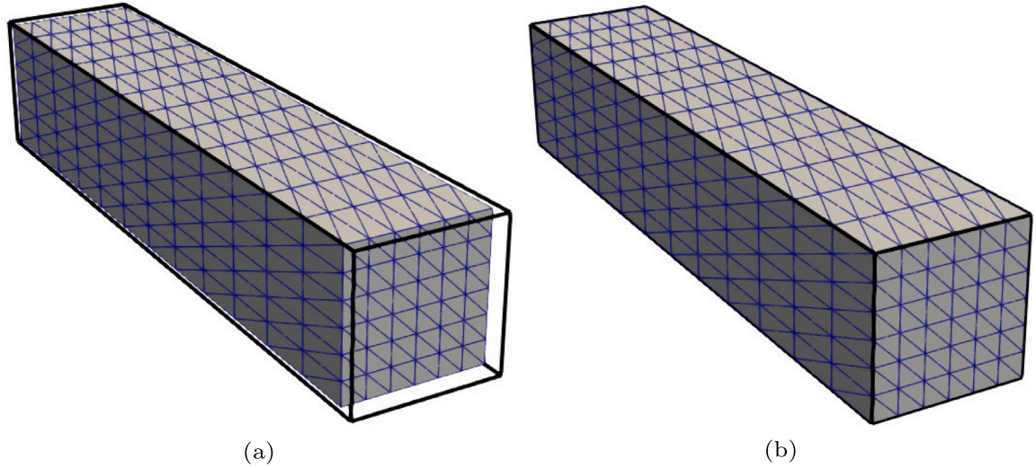
Fig. 3. Test 2, (a) the computed reference configuration with respect to the initial geometry (black contour). (b) the forward problem solution as computed starting from the reference configuration in (a).
